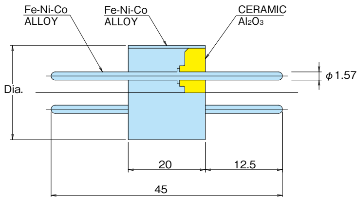
12PIN Φ22.2mm
